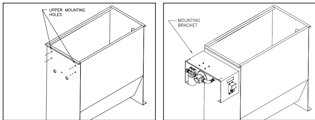
Fig. 7a & 7b: Installation of mounting bracket directly to power units only.
