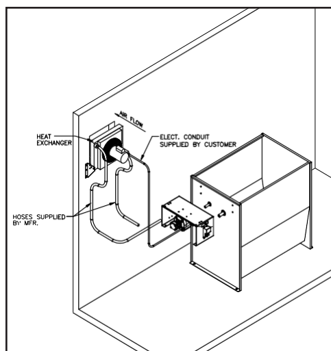
Fig. 3: Typical installation with wall mount of heat exchanger only.
