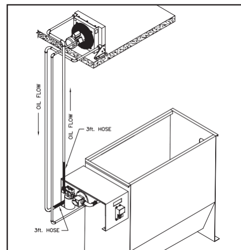
Fig. 4: Typical installation with (remote mount) of heat exchanger only.
